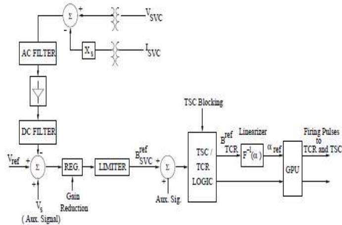
Figure 4:SVC Controller
