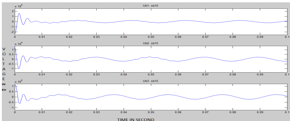
Figure 9: Voltage Waveform of Bus 10 without SVC
