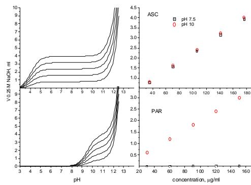
Figure 5- Potentiometric and calibration curves of PAR and ASC.
