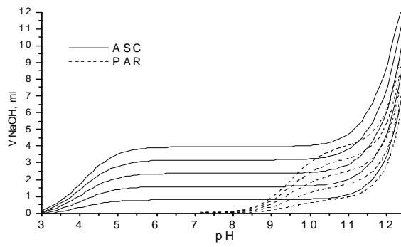
Figure 4- Overlapped pH peaks of PAR and ASC
