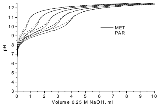
Figure 1 - Overlapped potentiometric curves of PAR and MET
