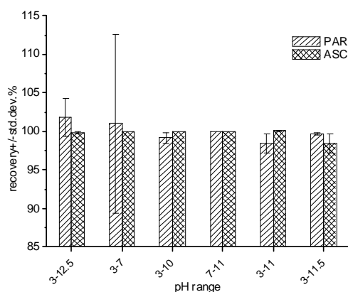
Figure 7- Recovery with error bar of PAR and ASC in binary mixtures using CLS method on different pH range
