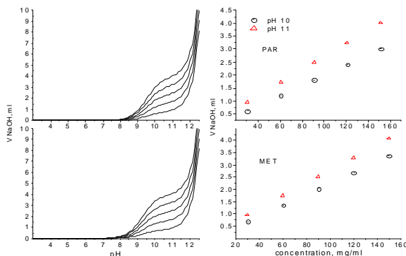
Figure 2- Potentiometric curves and their corresponding calibration curves of PAR and MET
