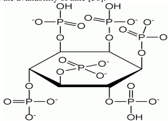
Figure 1. Structure of Phytate ( Insp_6 ), empirical formula= C_6P_6O_{24}H_{18}
